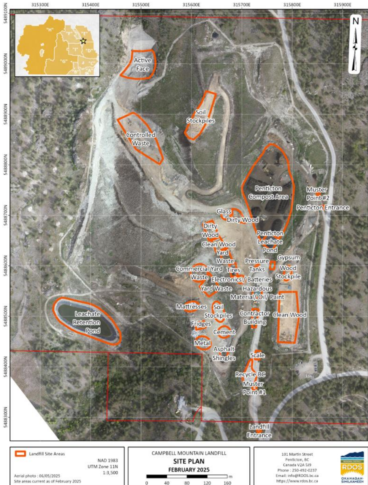
Figure 1: 2024 Campbell Mountain Landfill Site Plan
