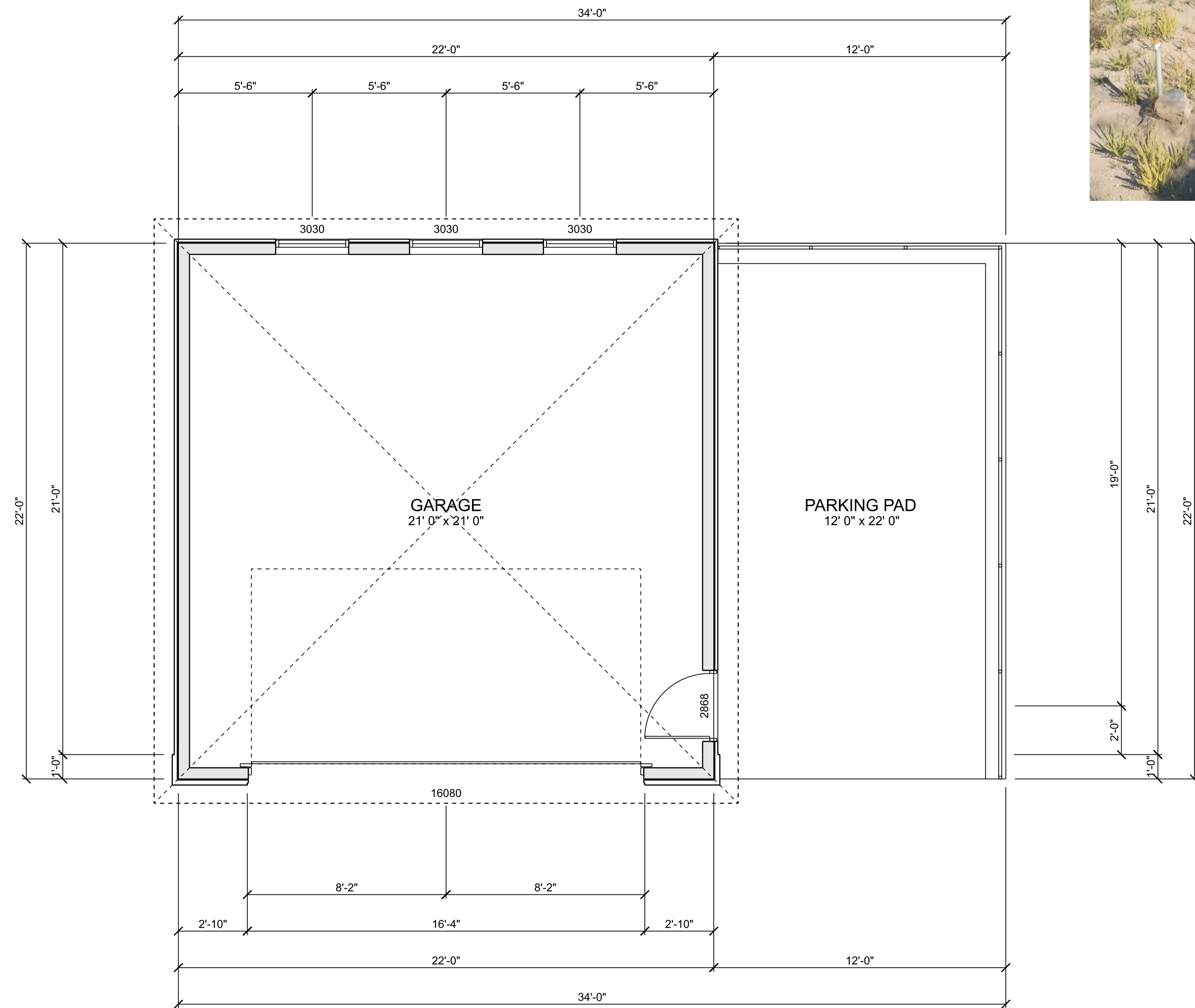
GARAGE PLAN SCALE: 1/4" = 1'-0" GARAGE AREA: 484 sq ft. PARKING PAD AREA: 264 sq ft.
