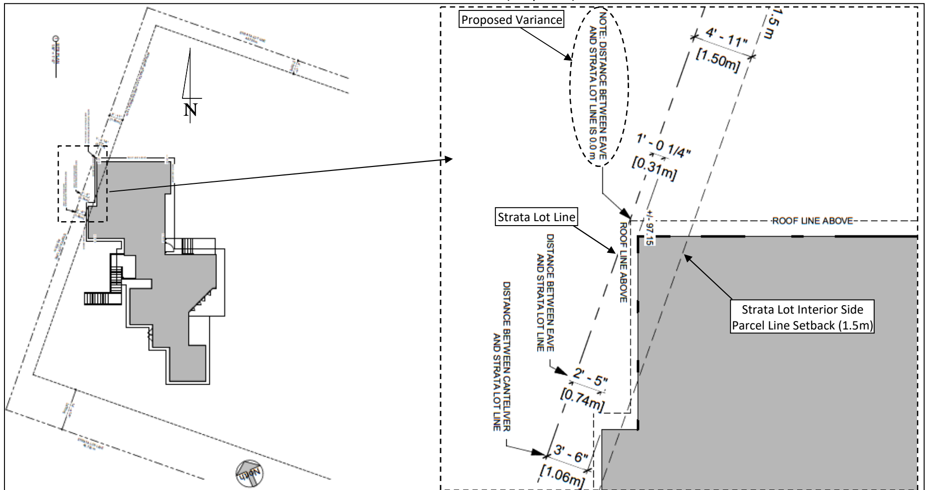
Schedule 'C' –Site Plan (Proposed)
