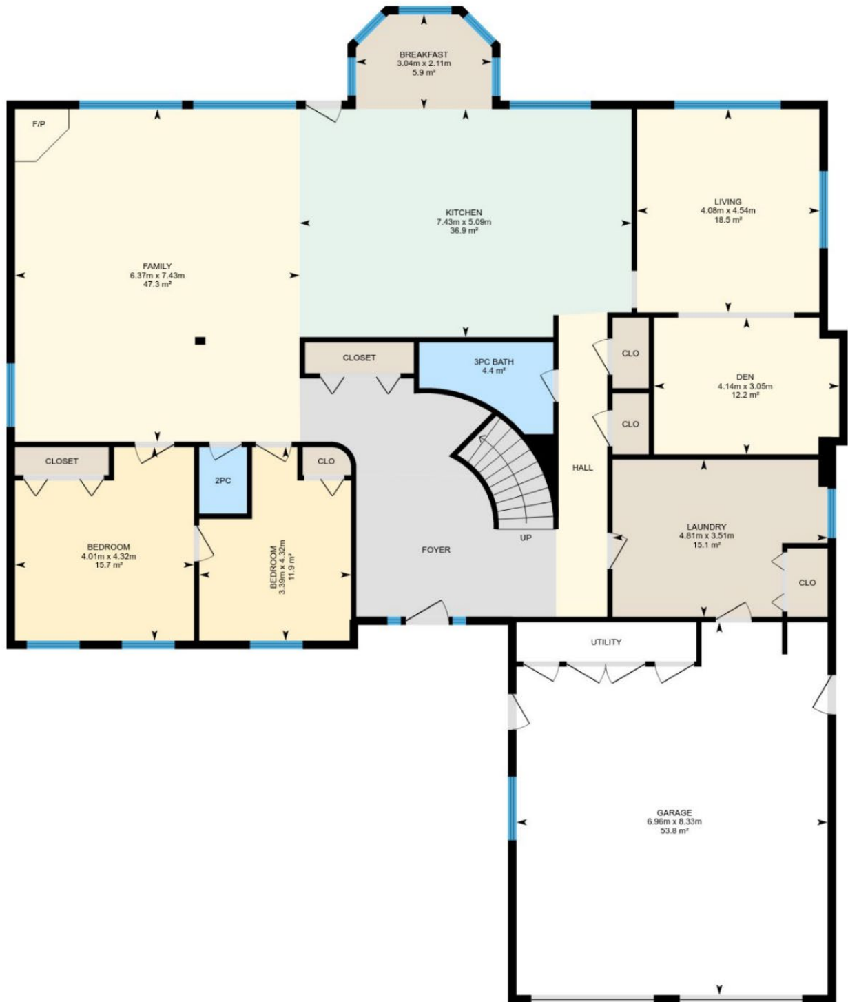
Figure 5 Subject Property Floor Plan - 1st Floor
