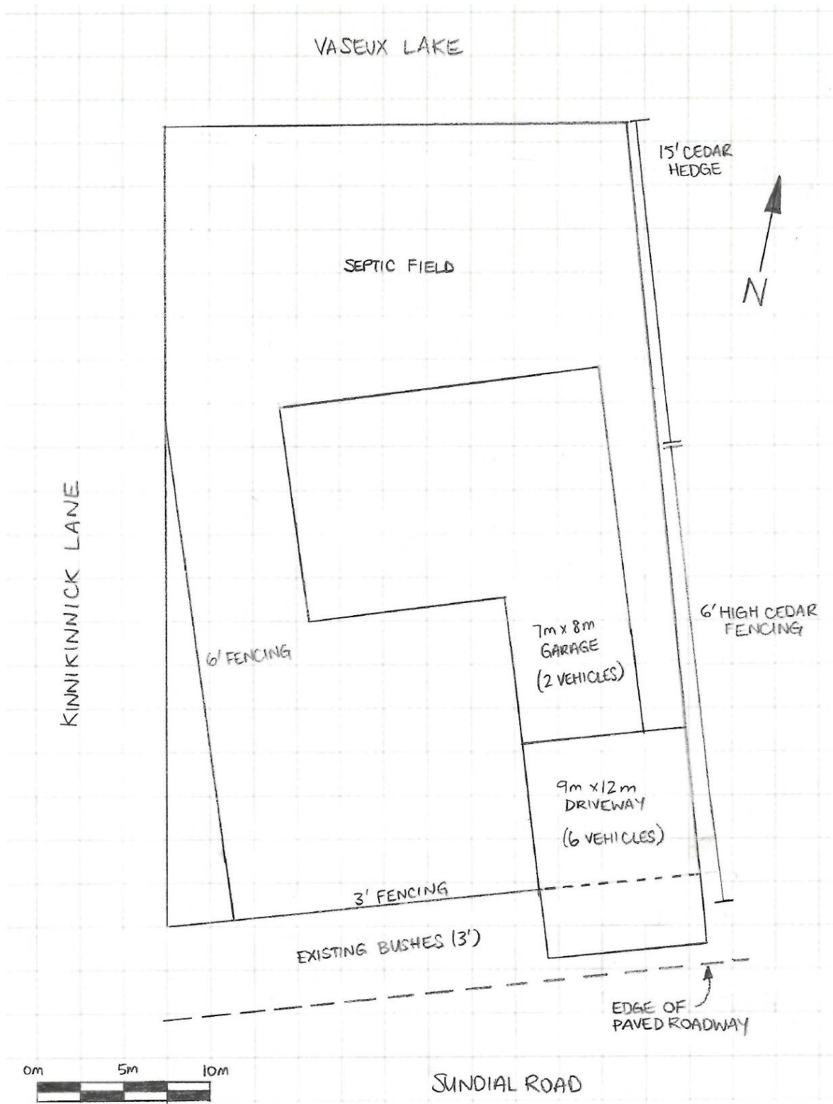
Figure 4 Subject Property Site Plan Detail
