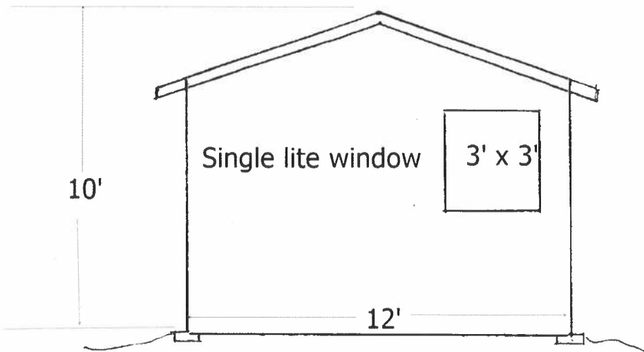
East (rear) Elevation
