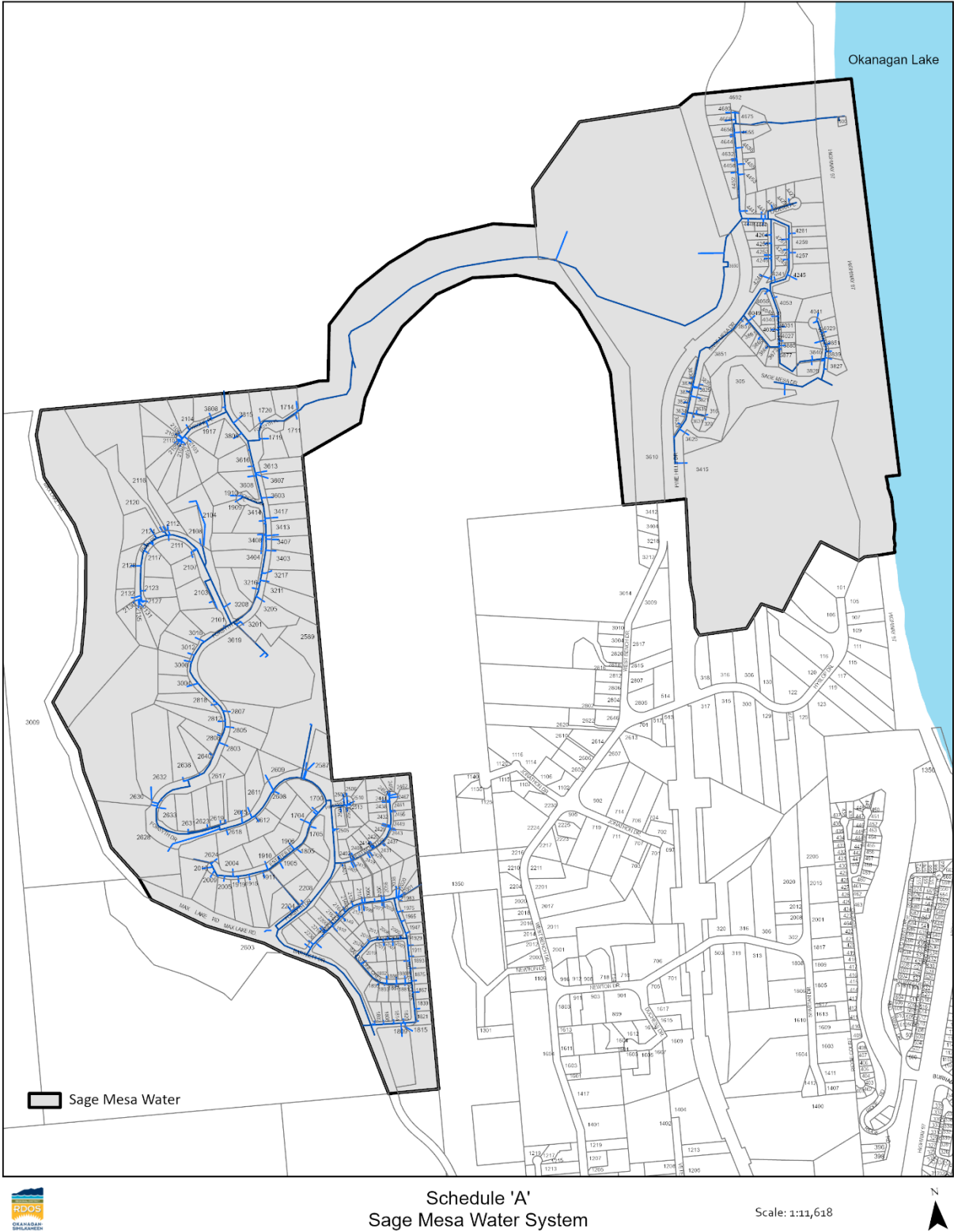
Figure 1: Sage Mesa water system servicing area.
