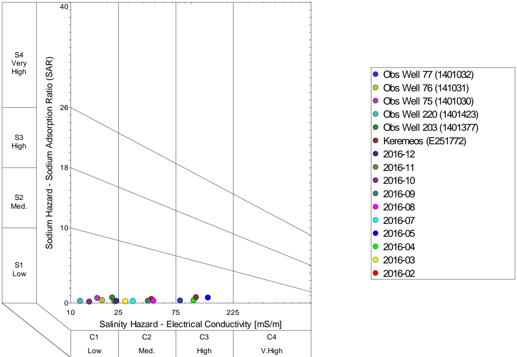
Figure D-4: SAR Diagram
