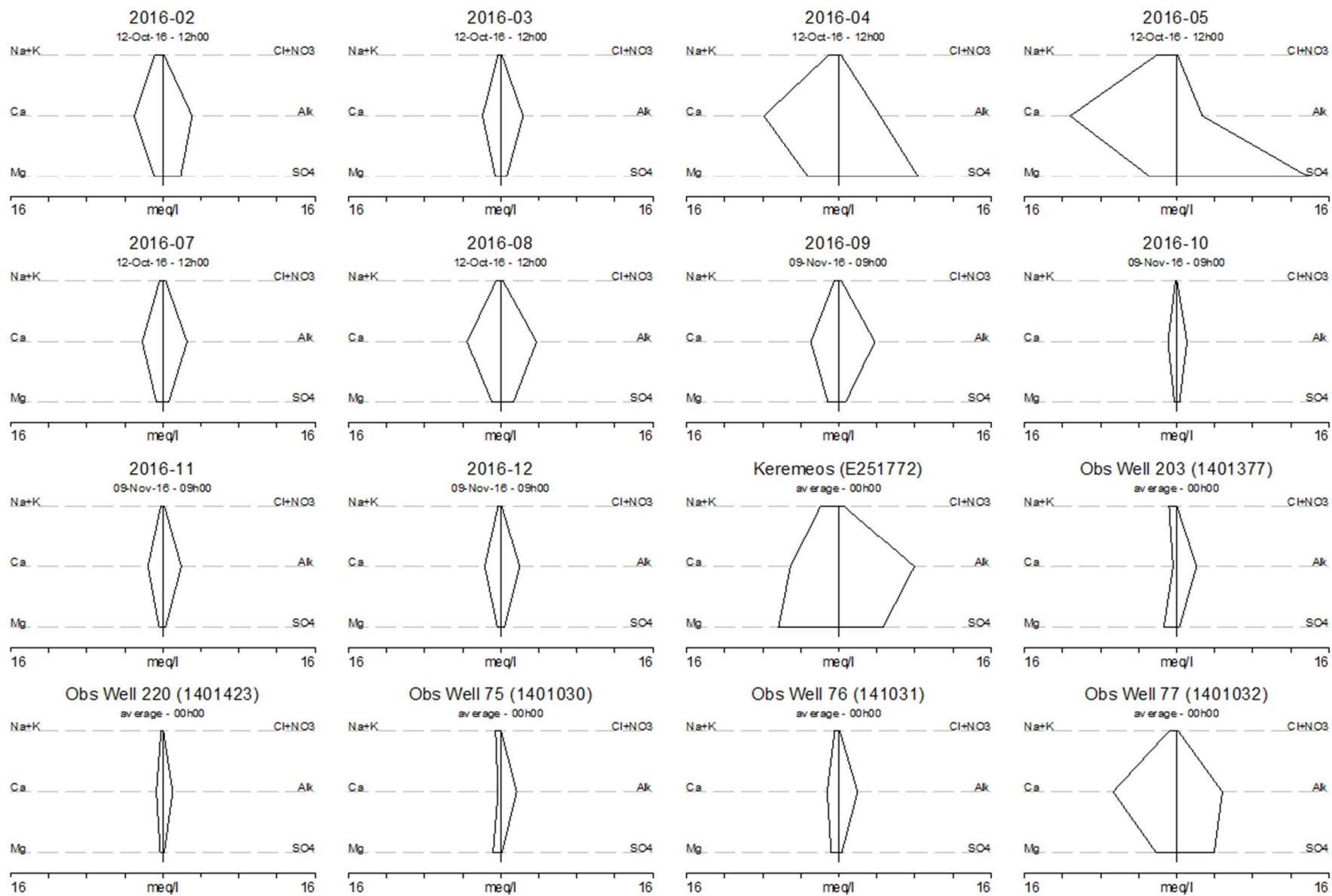
Figure D-3: Stiff Diagrams
