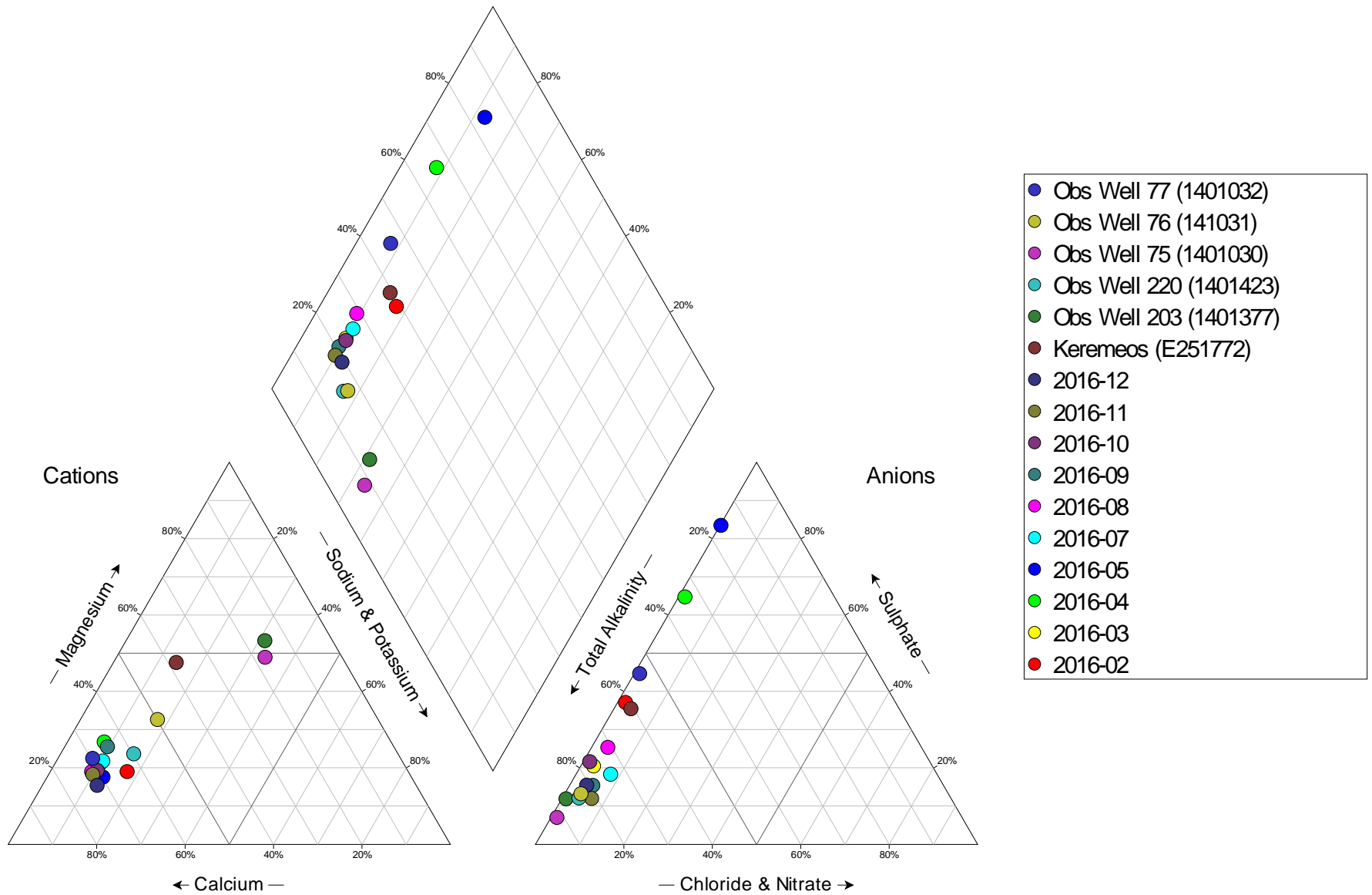
Figure D-1: Piper Diagram
