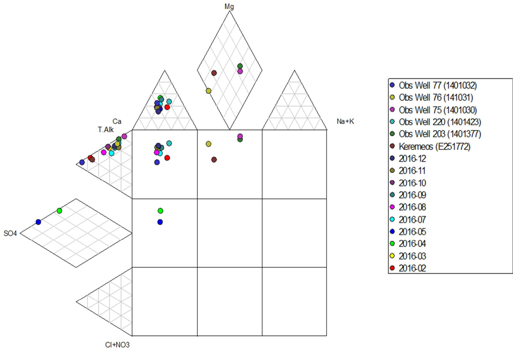
Figure D-2: Expanded Durov Diagram
