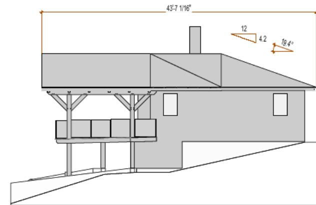
Elevation South-West
