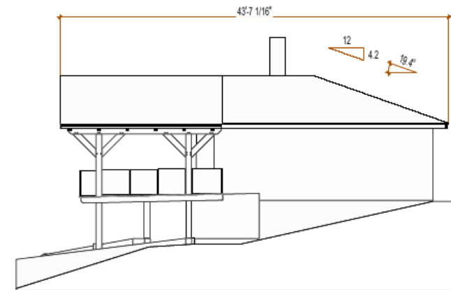
Elevation South-West
