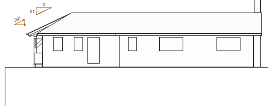
Elevation North-East
