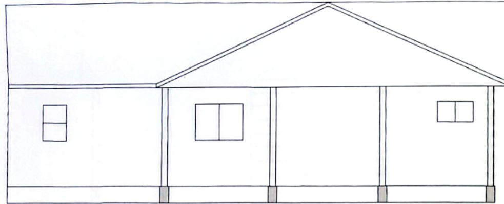
① EXISTING SOUTH ELEVATION 1/4" = 1' - 0"
