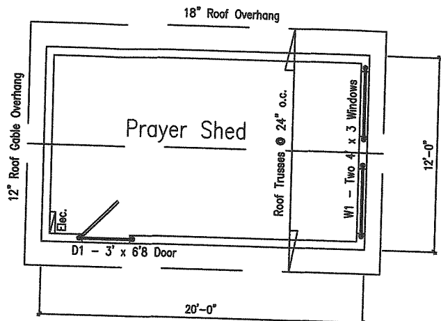
PRAYER SHED - FLOOR PLAN
