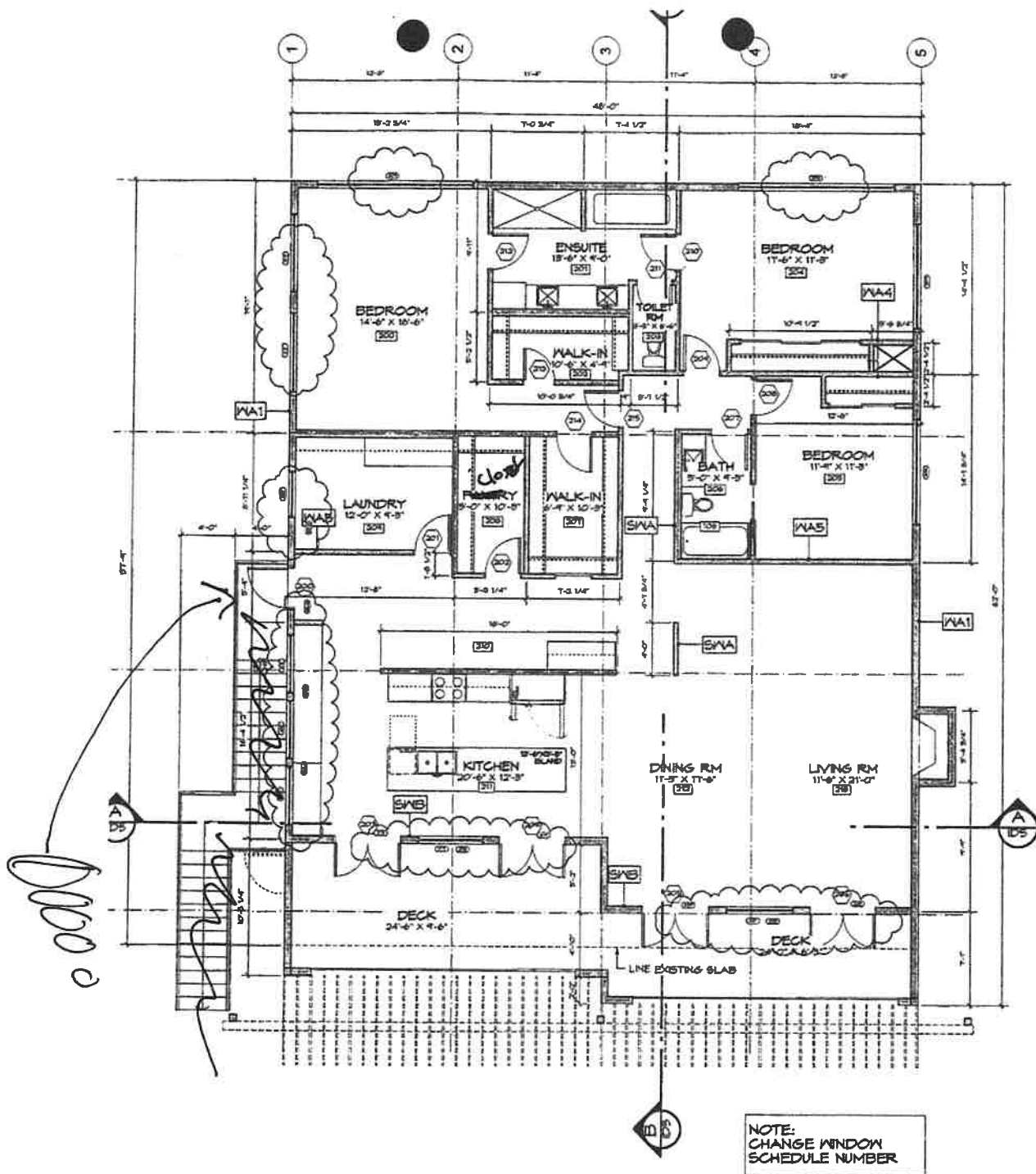
1 FLOOR PLAN
