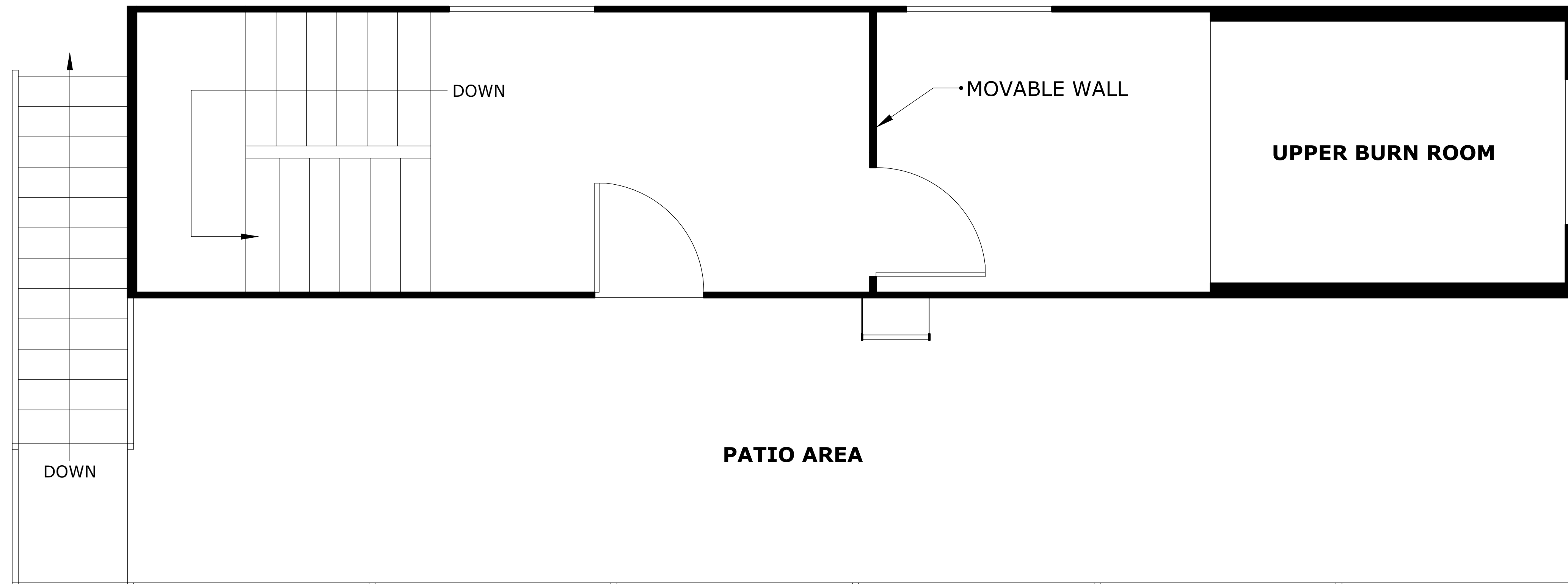
PLAN - UPPER
