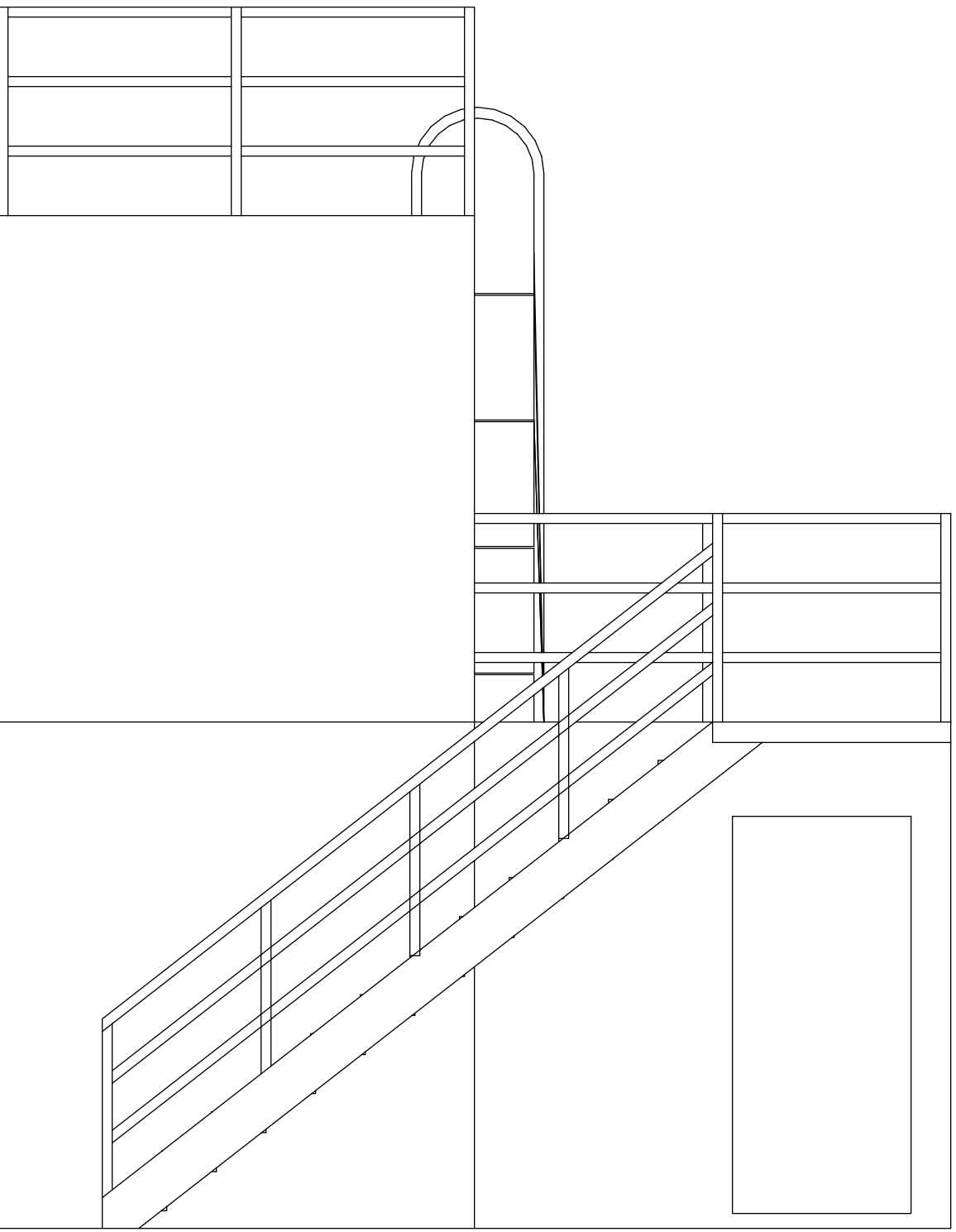
ELEVATION - SIDE (NORTH)
