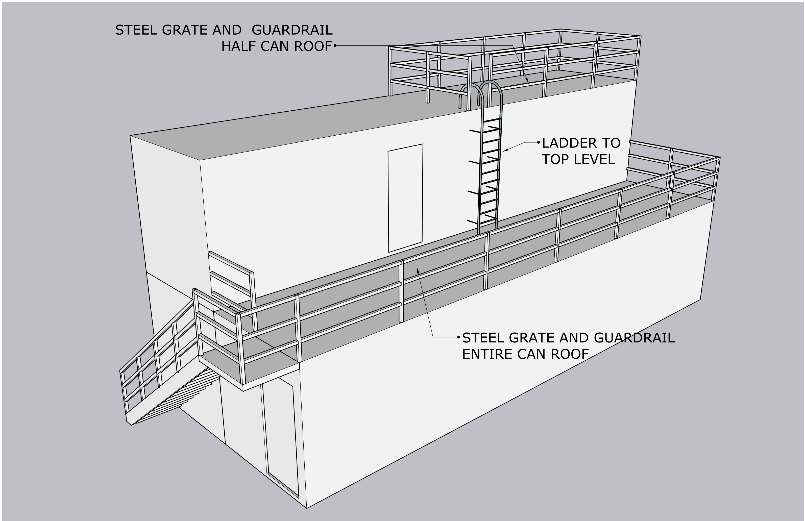
PERSPECTIVE - REAR
