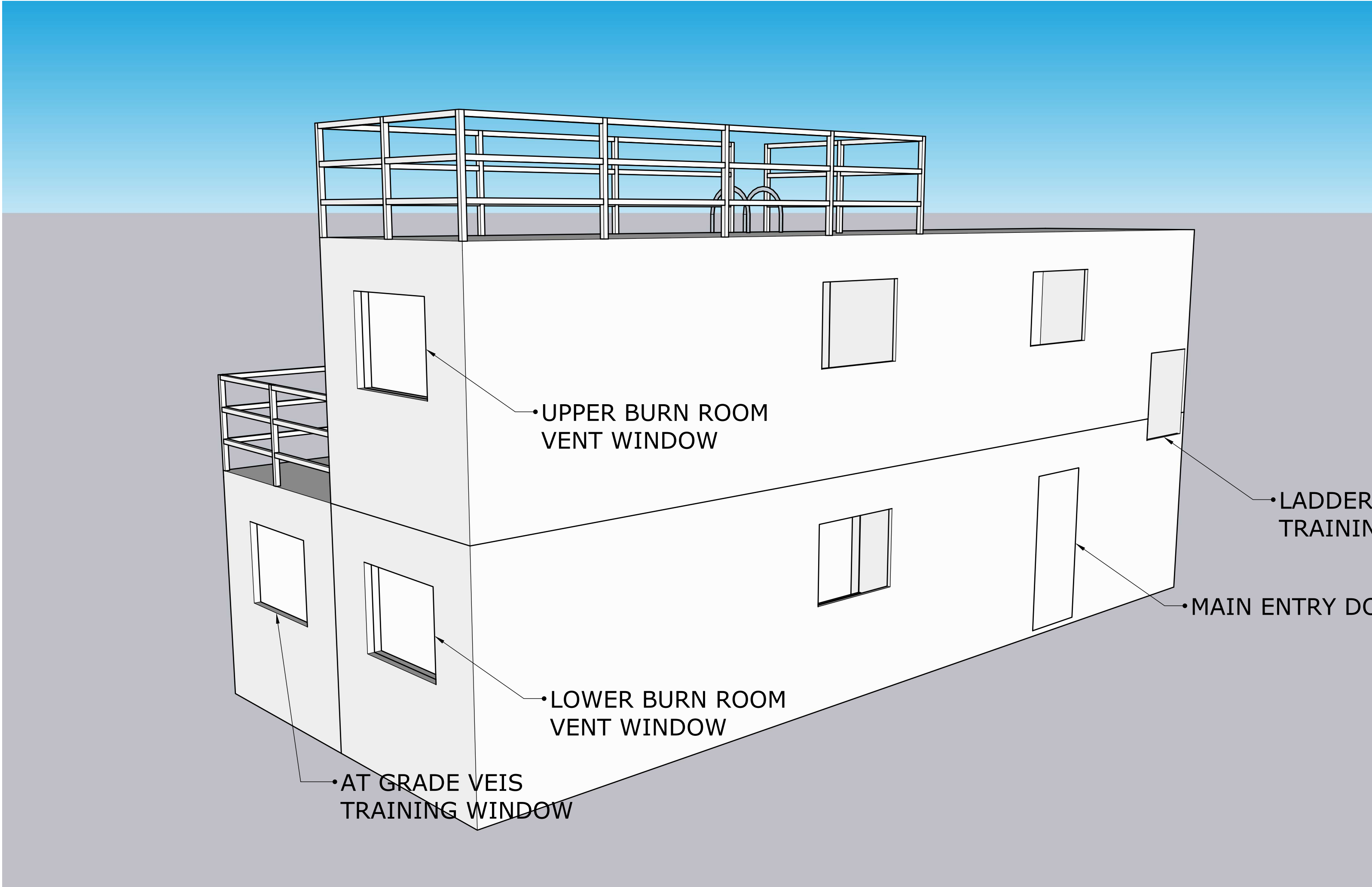
PERSPECTIVE - FRONT
