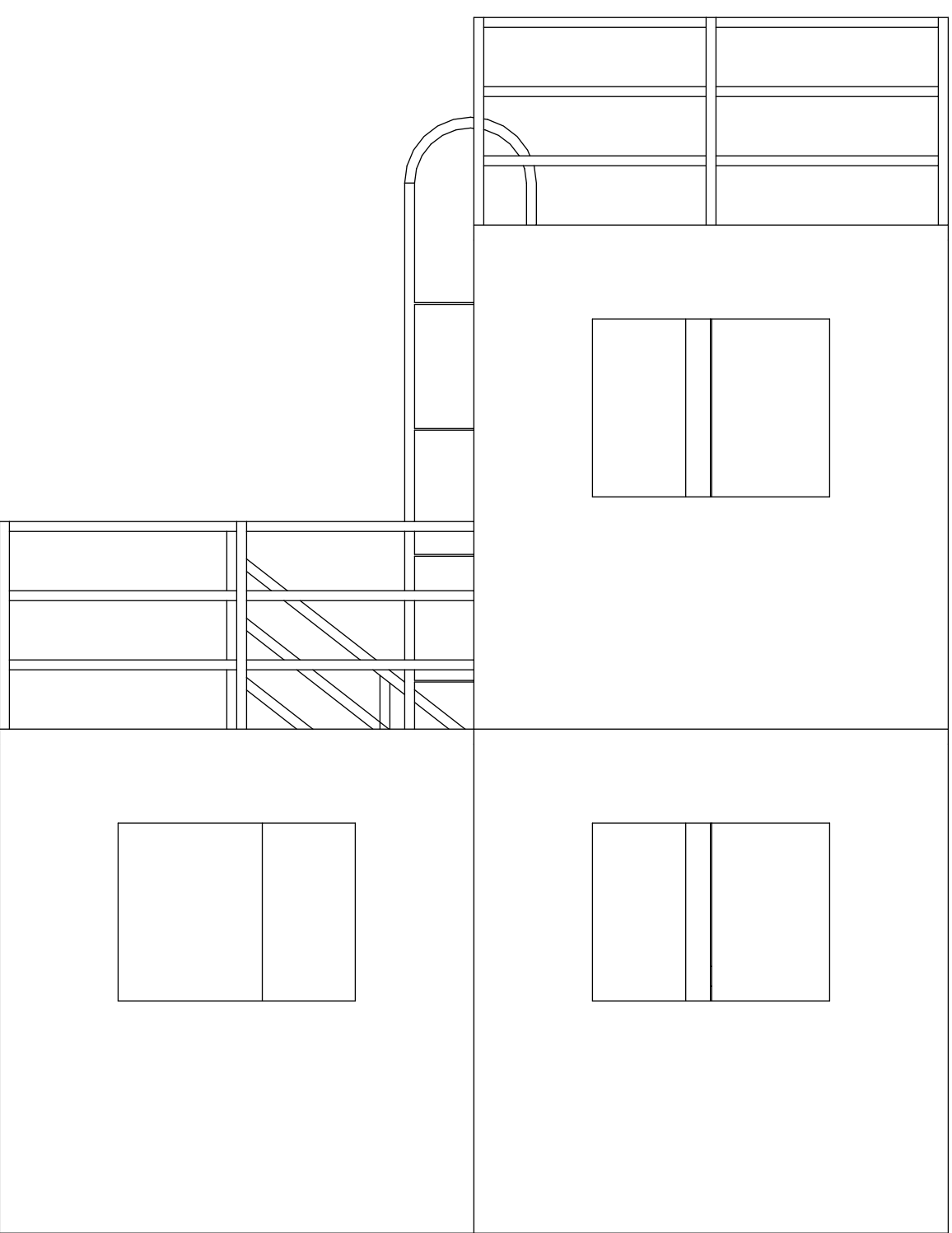
ELEVATION - SIDE (SOUTH)
